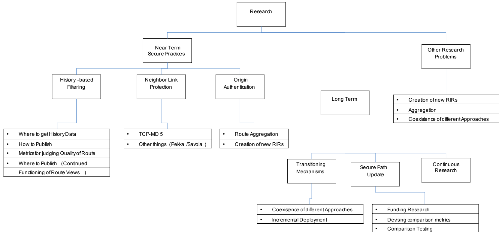
Figure 3: Research Roadmap.
